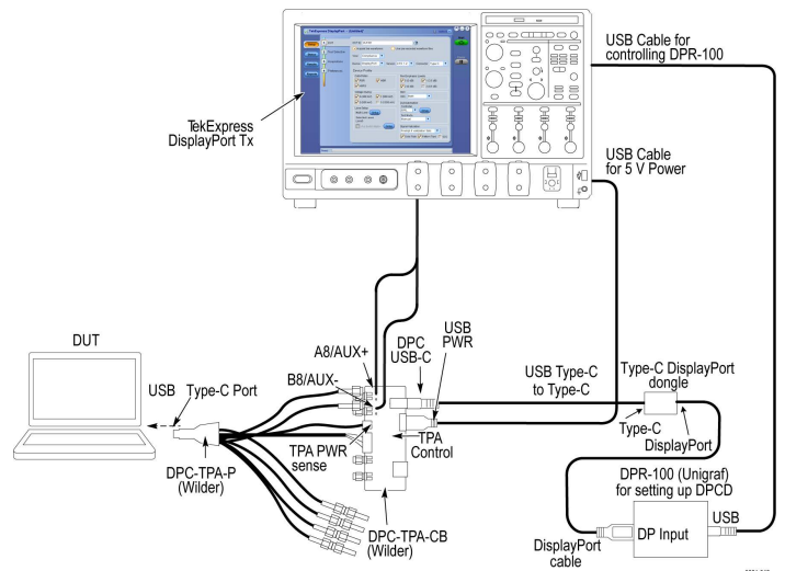
DisplayPort Type-C setup with dongle
