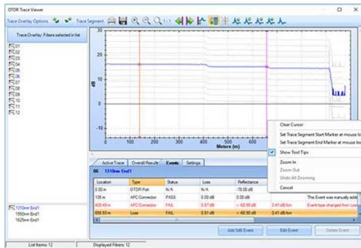
Setting span event parameters using LinkWare PC
