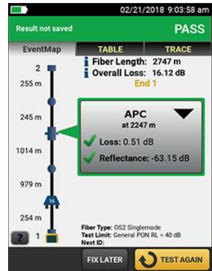
Event modified to be an APC connector
