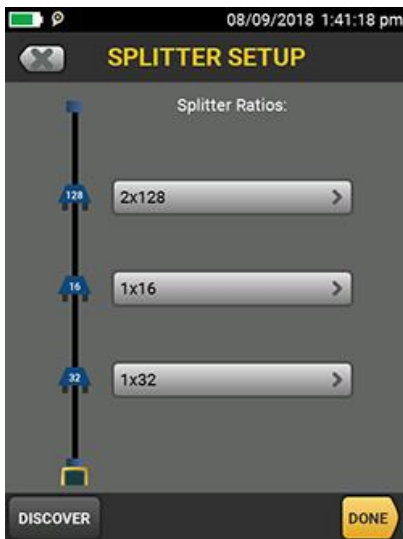
Splitter setup
