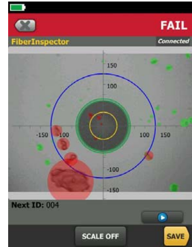
FiberInspector probe
