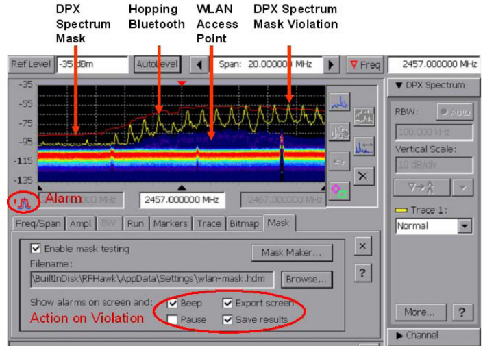
DPX Spectrum Mask captures and logs spectrum violations with options of warning alarm, pausing test, export screen, and result save
