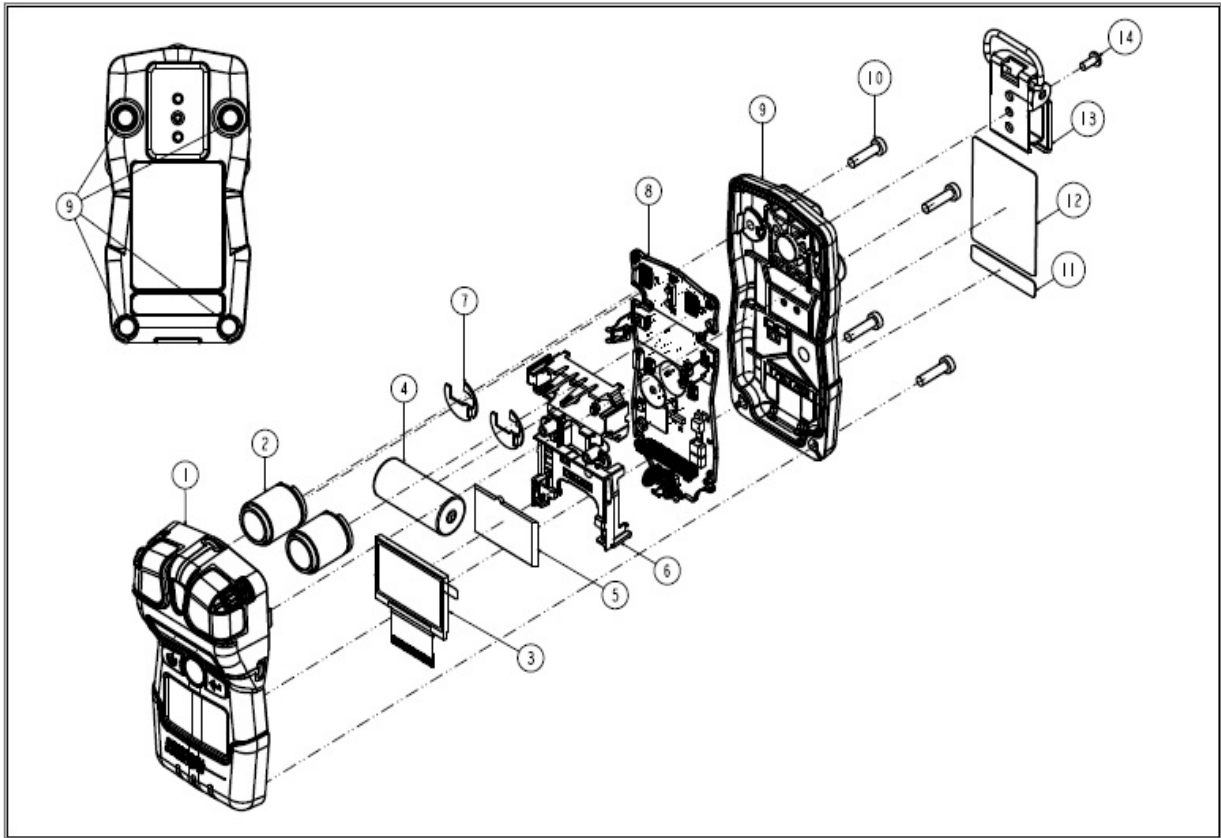
Figure 6.1 Disassembled Tango TX1
