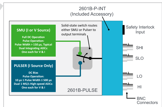
External Interlock/Connector box included with 2601B-PULSE
