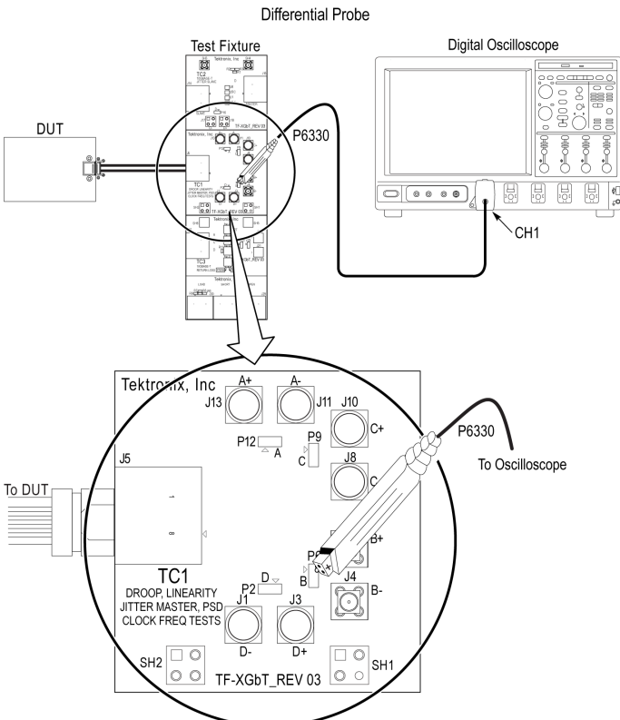
Connection diagram
