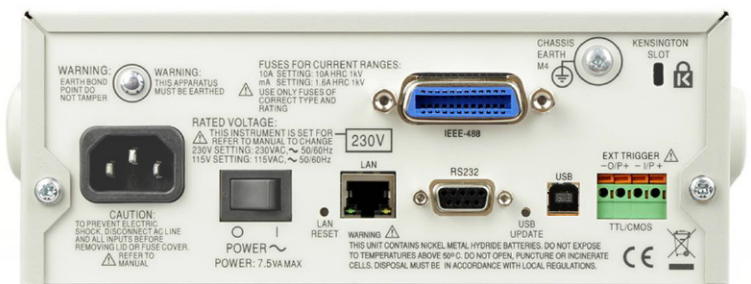
1908P rear panel (protective buffer removed)
