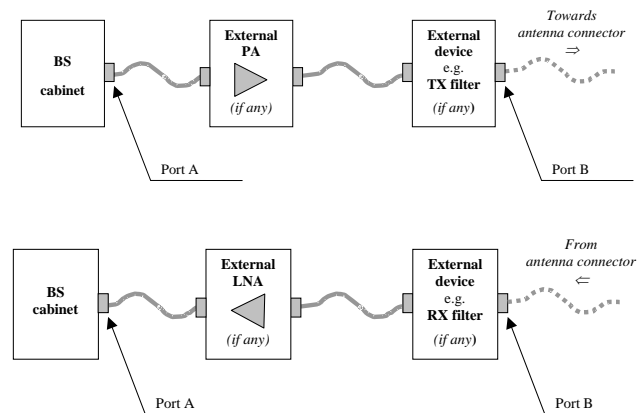
Figure 1: BS type 1-C transmitter receiver interface [1]
