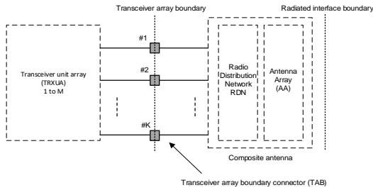
Figure 2: Radiated and conducted reference points for type 1-H [1]
