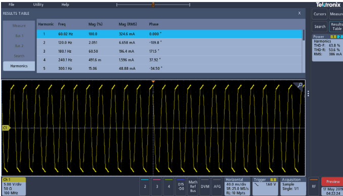
Figure 10. Harmonics Analysis.
