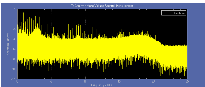
Transmitter Spectral Profile for Common Mode Analysis
